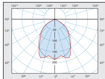
Intensity distribution in cd/1000lm
